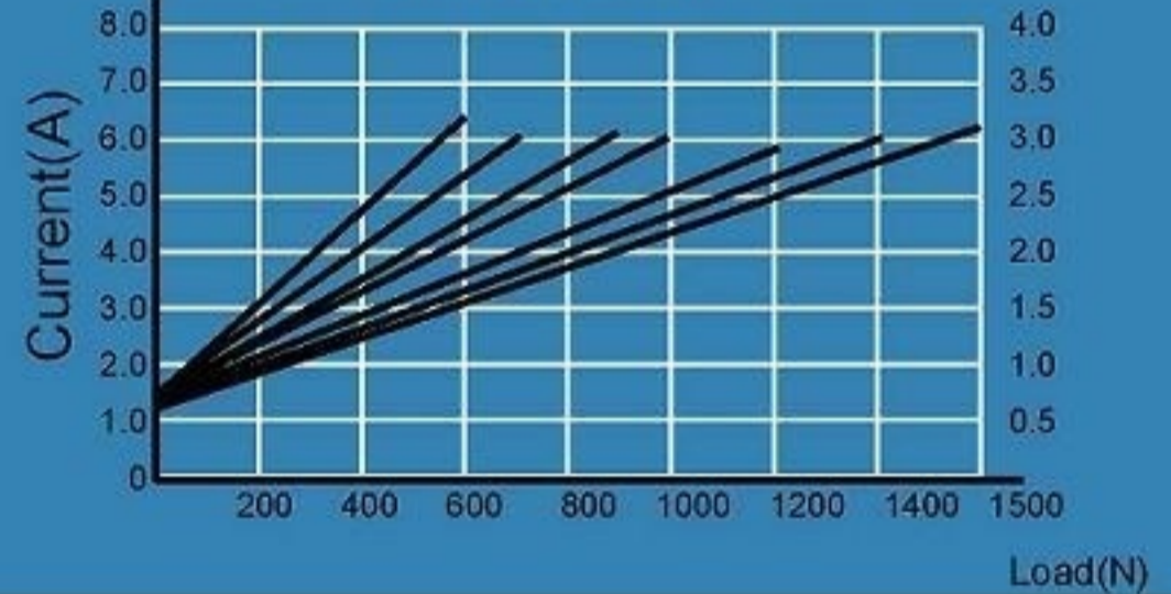
Current-Load
